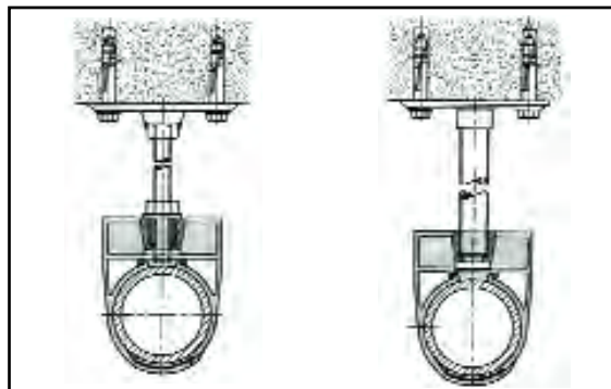
Clíc 63-113 fixing possibilities
