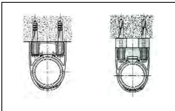
Clíc 8-59 fixing possibilities
